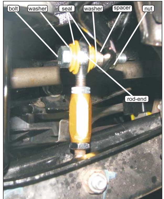
Fig 1 - KLC066 left side, rear view.
