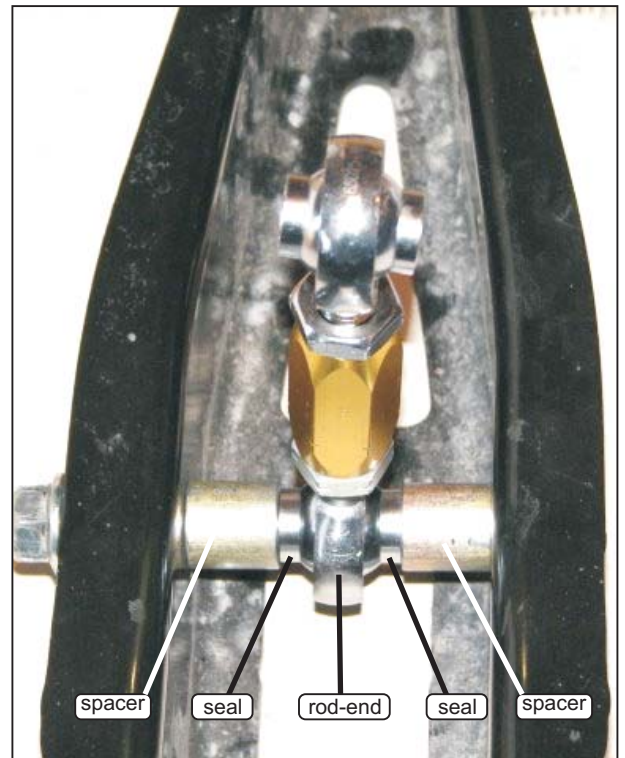
Fig 2 -KLC066 control arm mount (rod-end seals not shown).
